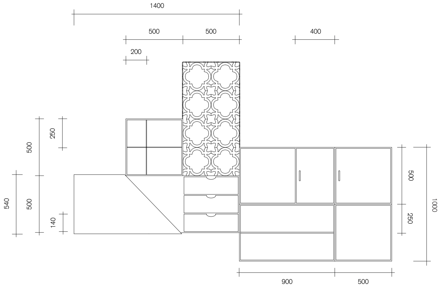
FRONT
